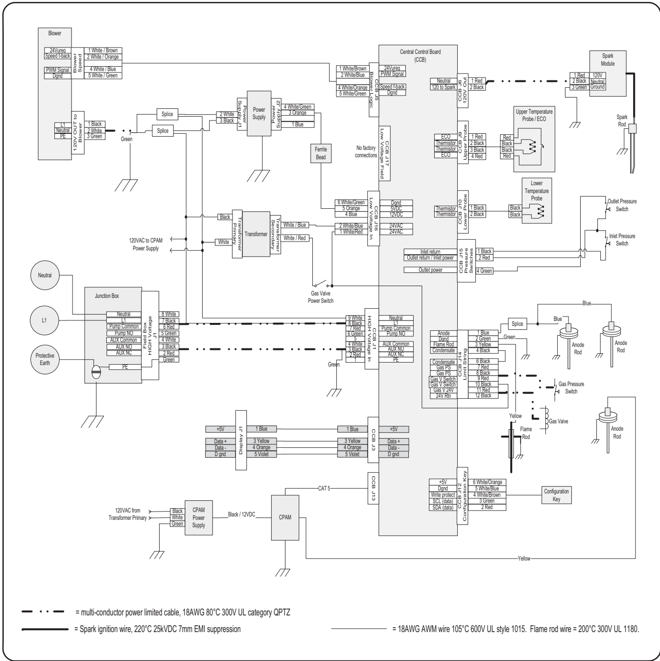
Figure 67. Wiring Diagram
