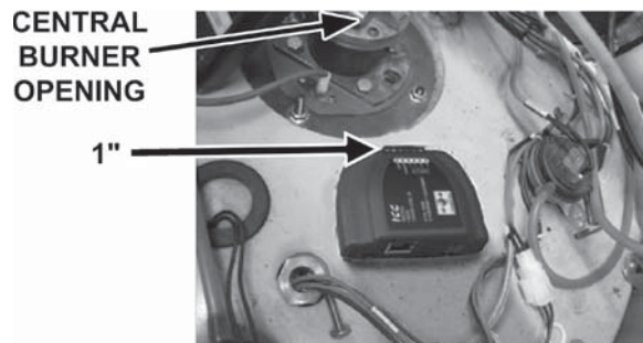
Figure 24. Locating Upper Temperature Probe and Exhaust Switch
