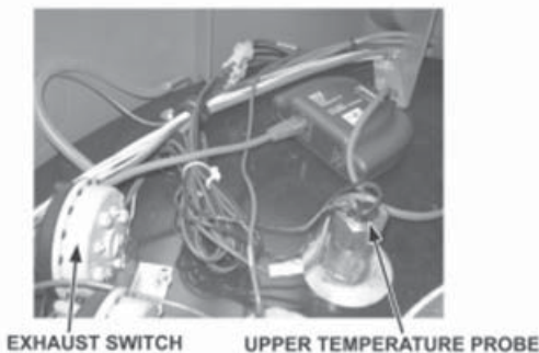
Figure 15. Location of Exhaust Switch and Upper Temperature Probe
